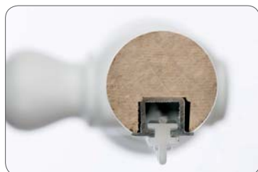
Pole Cross Section
